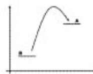
endotherm
