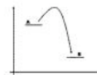
exotherm
